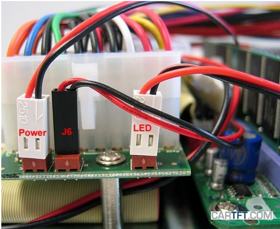
The black/red cable (J6) gets connected this way:
